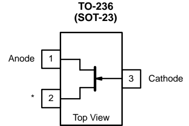
*Short lead #2 to Cathode (lead #3) via circuit board trace.
